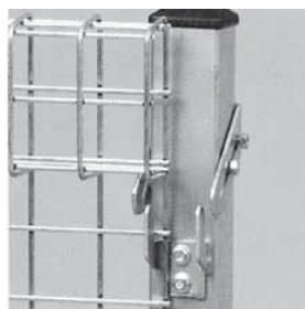
SLIDE AND LOCK MECHANISM WITH FIXING LUGS
