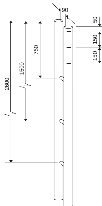
GATE - DOUBLE POST
