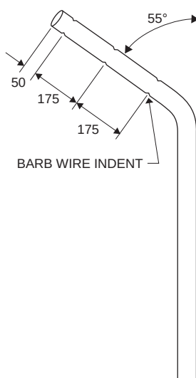
CORNER CRANKED POSTS
